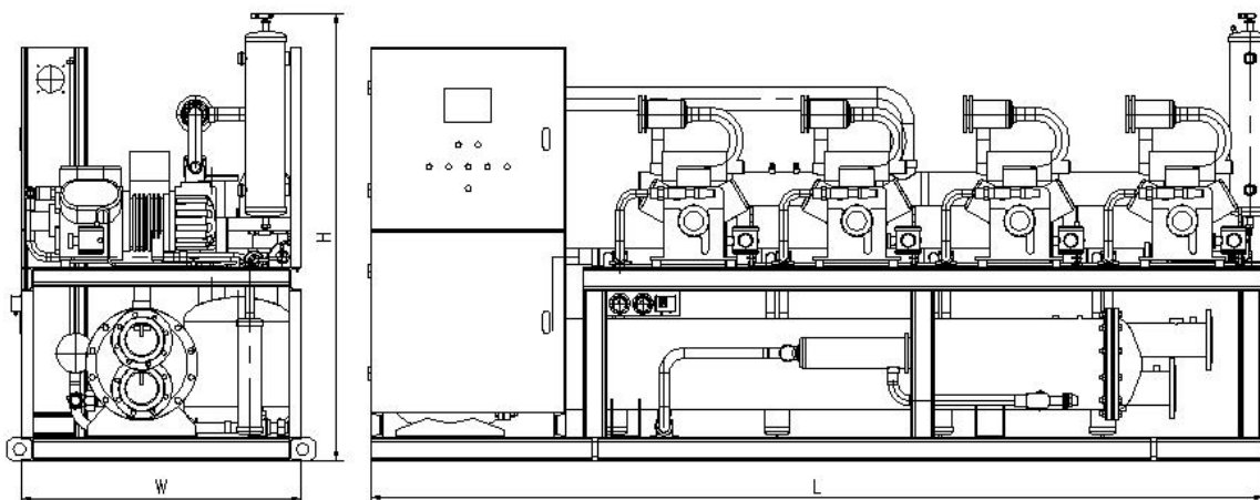
4 Compressor racks
