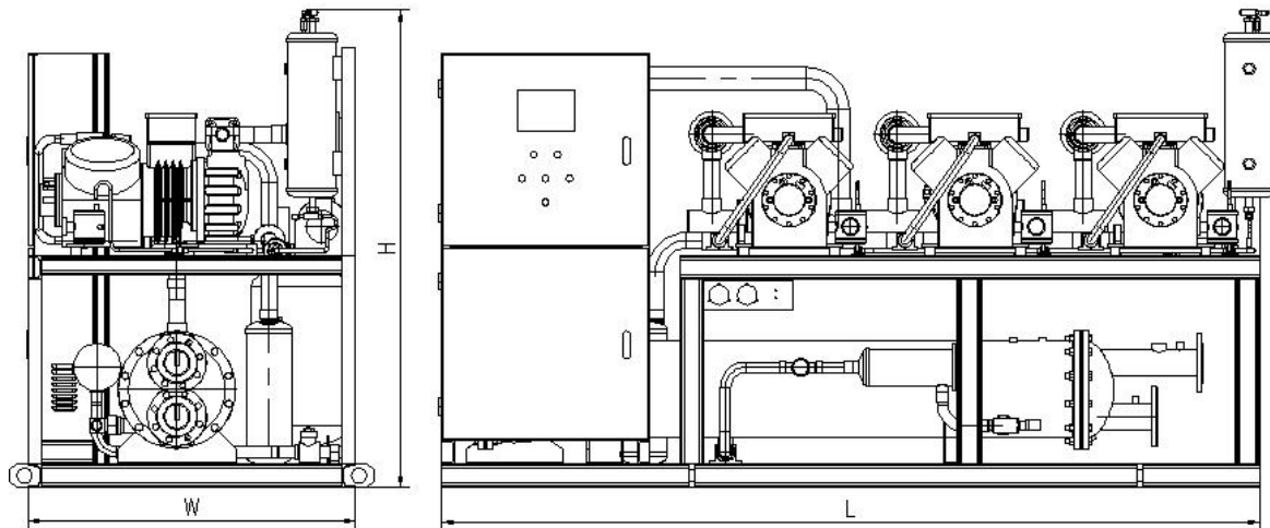
4 Compressor racks
