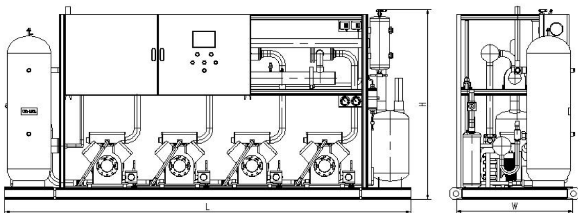
4 compressor racks
