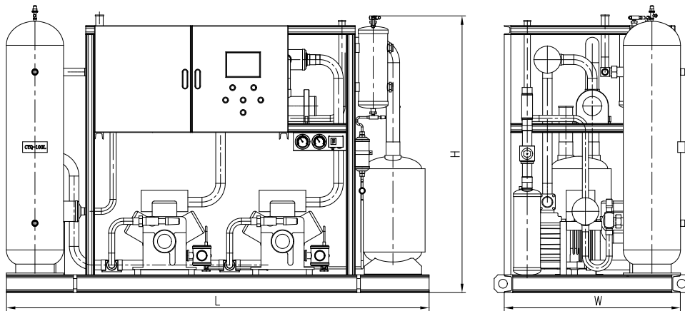
2 compressor racks
